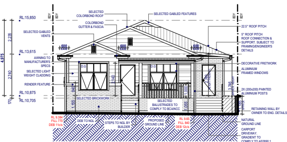
FRONT - WESTERN ELEVATION
