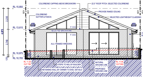
REAR - EASTERN ELEVATION
